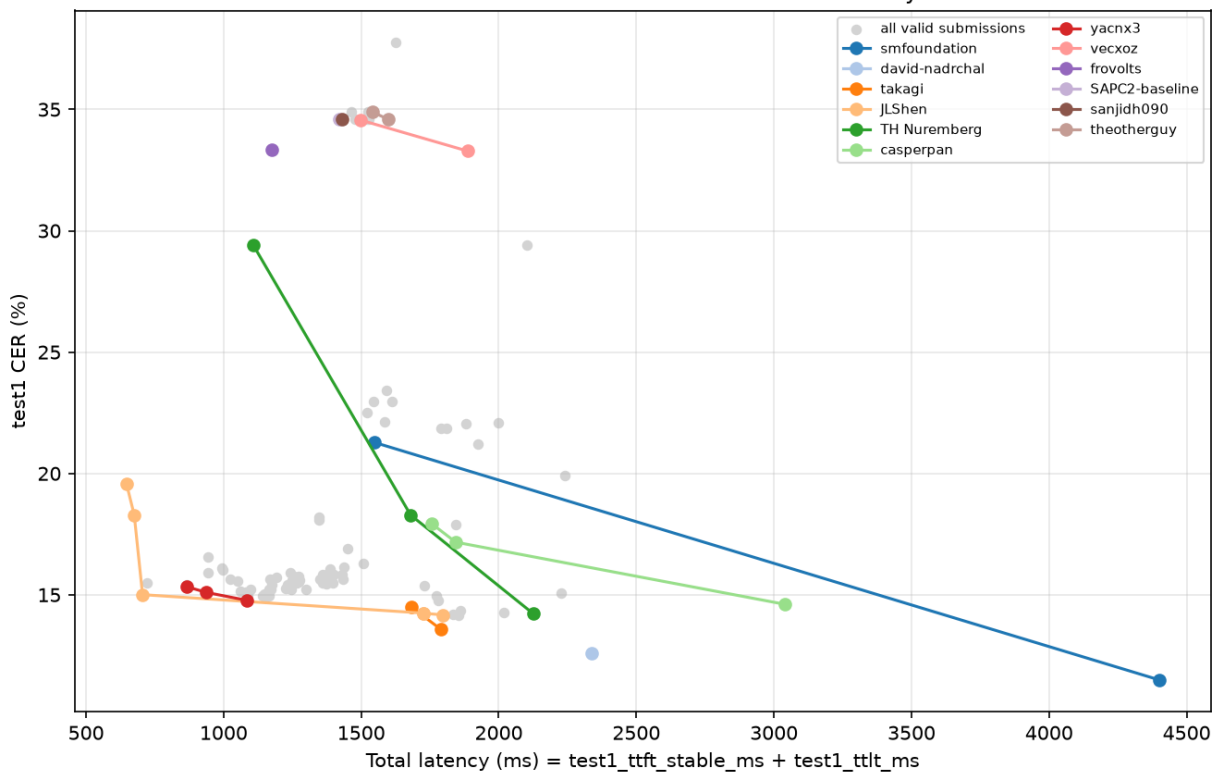
Team Pareto frontier: test1 CER vs. total latency
